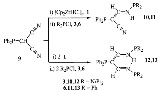
Scheme 3. Mono- and dihydrozirconation/transmetalation reactions of the phosphanylmalononitrile compound 9
