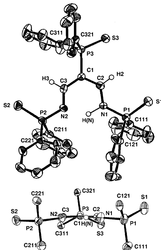
Figure 3. Two views of the molecular geometry of Ph_2P(S)C[CHNP(S)Ph_2]_2(\mu-H) ( 14 ) as determined by X-ray diffraction
