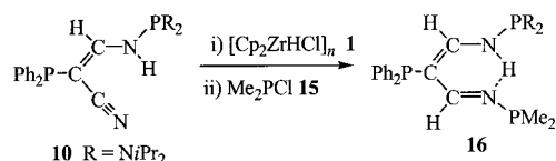
Scheme 4. Monohydrozirconation/transmetalation reactions of the phosphanyl- \beta -nitriloeneamine compound 10
