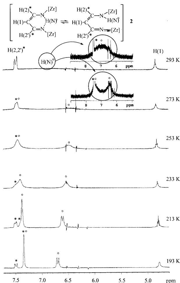
Figure 1. 1D selective TOCSY of 2 at variable temperature with excitation of \text{H}(1) (the corresponding symmetric Lewis structures are omitted for clarity); mixing time = 60 ms; [\text{Zr}] = \text{ZrCp}_2\text{Cl}
