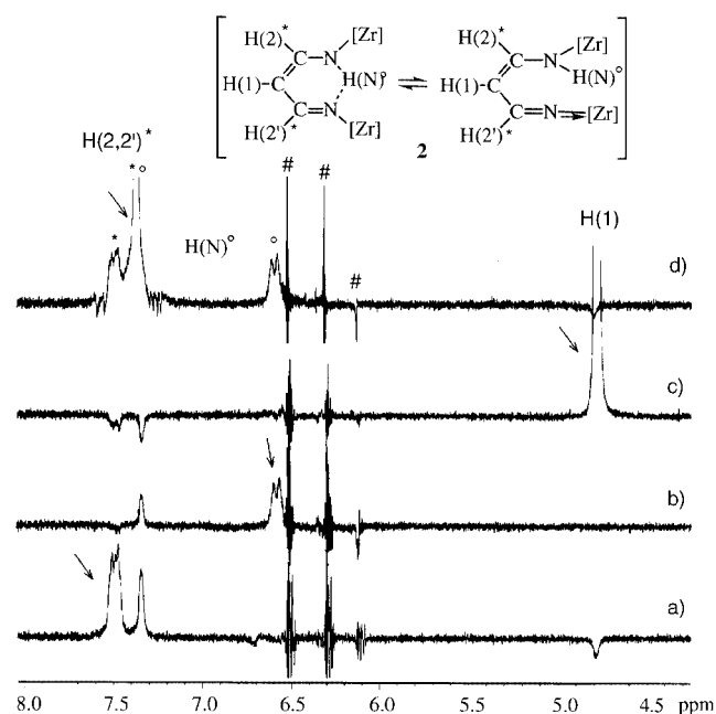
Figure 2. 1D GROESY of 2 at 193 K (the corresponding symmetric Lewis structures are omitted for clarity) with selective excitation of the site indicated by the arrow \rightarrow ; mixing time = 200 ms; lines denoted by # are residual signals of the Cp protons; [\text{Zr}] = \text{ZrCp}_2\text{Cl}
