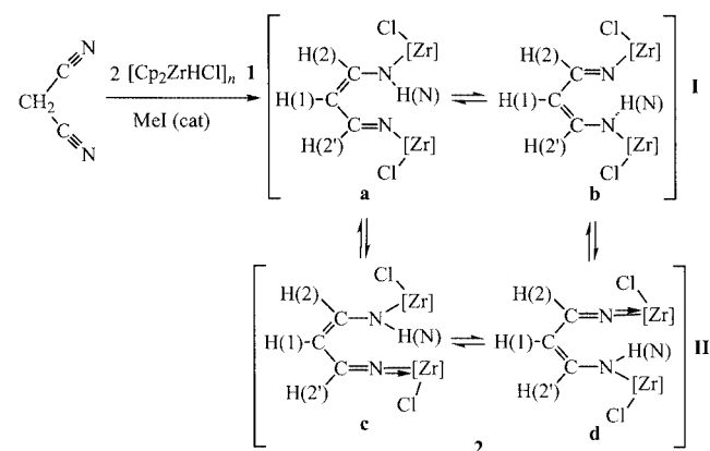
Scheme 1. Description of the different conformers of the ( N -zircona- \beta -enamino)imine derivative 2 at 193 K; [Zr] = ZrCp_2
