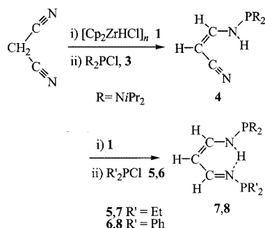
Scheme 2. Selective monohydrozirconation/transmetalation reactions of malonodinitrile and the \beta -nitriloeneamine compound 4
